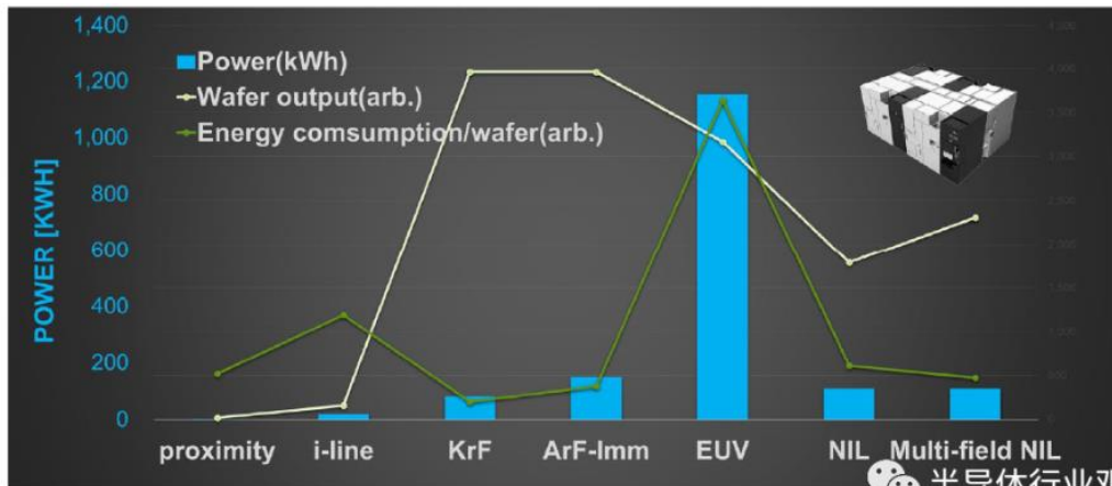
Figure 11. Energy consumption in lithography process and the estimation of an energy consumption for NIL.
