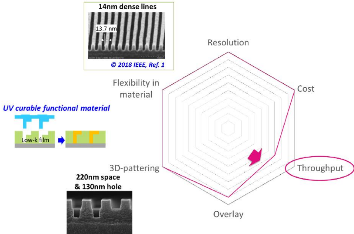
Figure 2. Current performance of NIL. 头条@半导体行业观察
