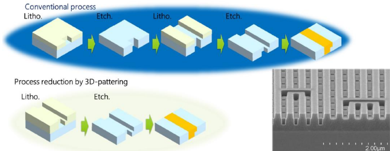
Figure 12. Concept to reduce process steps with 3D-patterning of NIL.
