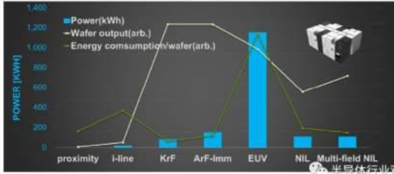
Figure 11. Energy consumption in lithography process and the estimation of an energy consumption in NIL. 20
