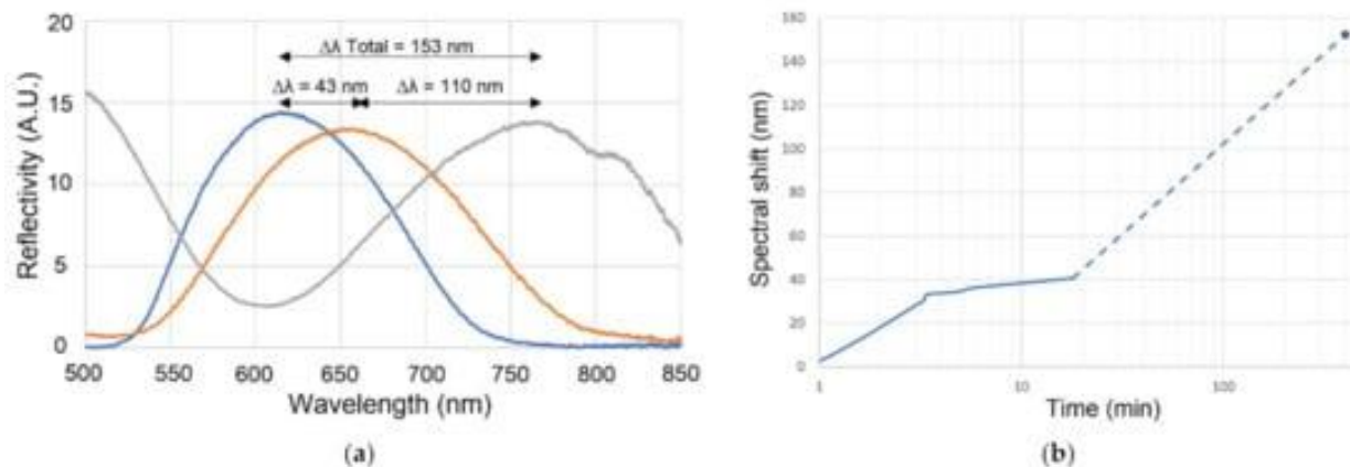
Figure 6. Sensing performance of a F127-templated mesoporous TiO 2 Fabry-Pérot structure. (a) Evolution of the optical reflectance spectrum of the sensing sample under a water environment after the first 18 h (orange color) and after additional 17 days (gray color). The reflectance spectrum at the beginning of the sensing experiment is depicted in blue color. (b) Evolution with time of the position of the maximum in the optical reflectance spectrum during the initial sensing experiment lasting 18 h and after additional 17 days (only one measurement is acquired after that period).
