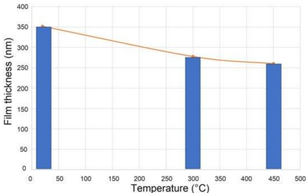
Figure 3. Evolution of the thickness of mesostructured F127-templated \text{TiO}_2 films, measured by profilometry, for increasing temperatures during the calcination process.
