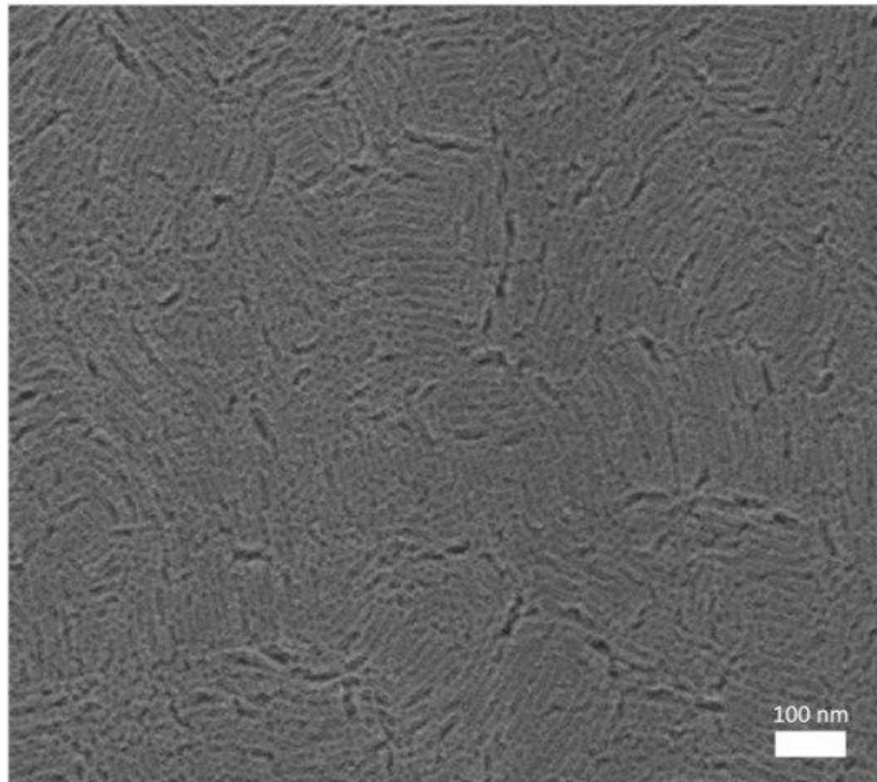
Figure 7. HRFESEM image of a P123-templated mesoporous \text{TiO}_2 film.
