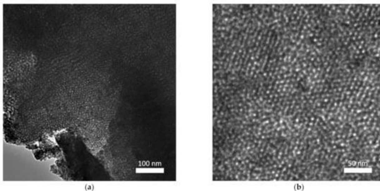
Figure 4. (a) TEM image acquired from a F127-templated mesoporous \text{TiO}_2 film after thermal treatment at 450 °C. (b) TEM image from the same sample and area, using a higher magnification to show the pore arrangement.
