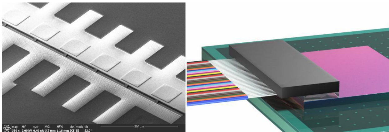
Picture: Nanoimprint of wafer-level optics on silicon photonics wafer (left) for Teramount PhotonicPlug's scalable fiber connectivity (right).
