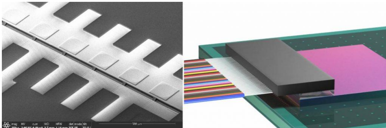
Nanoimprint of wafer-level optics on silicon photonics wafer (Left) for Teramont PhotonicPlug's scalable fiber connectivity (Right).
